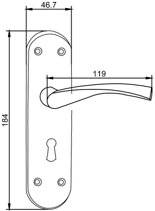
Lock
